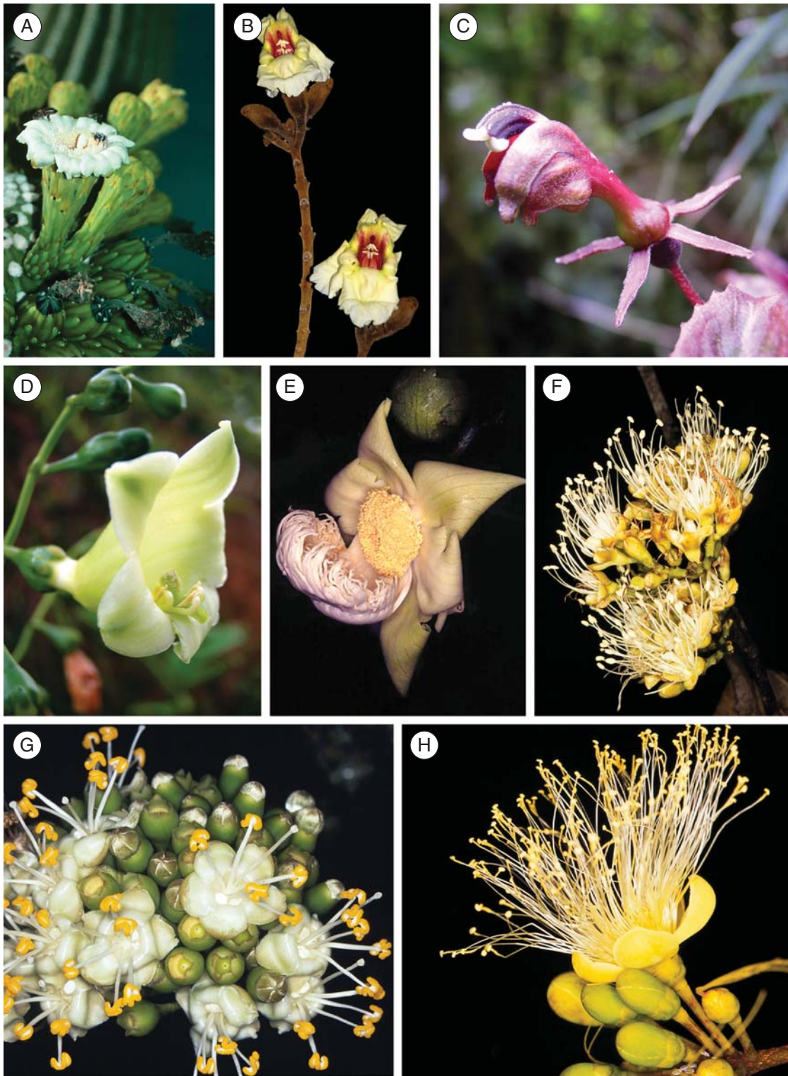
FIG. 4. Bat-pollinated flowers, their corolla or perianth length (when known), and their pollinators. (A) Carnegia gigantea (Caryophyllales: Cactaceae), corolla 112 mm, opportunistic and specialized phyllostomid bats; (B) Markhamia stipulata (Lamiales: Bignoniaceae), specialized pteropodid bats; (C) Burmeistera ceratocarpa (Asterales: Campanulaceae), corolla 13.2 mm, glossophagine bats; (D) Chelonanthus alatus (Gentianales: Gentianaceae), corolla 30–45 mm, glossophagine bats; (E) Lecythis poiteaui (Ericales: Lecythidaceae), androecium 50 mm, glossophagine bats; (F) Hymenaea courbaril (Fabales: Fabaceae), flower diameter 25 mm, opportunistic and specialized phyllostomid bats; (G) Ceiba pentandra (Malvales: Malvaceae), flower diameter 25–35 mm, opportunistic and specialized phyllostomids and pteropodids; (H) Caryocar glabrum (Malpighiales: Caryocaraceae), flower diameter 40 mm, opportunistic and specialized phyllostomid bats. Photo credits: T. Fleming (A, B), C. Geiselman (D), S. Mori (E–H), N. Muchhala (C).
