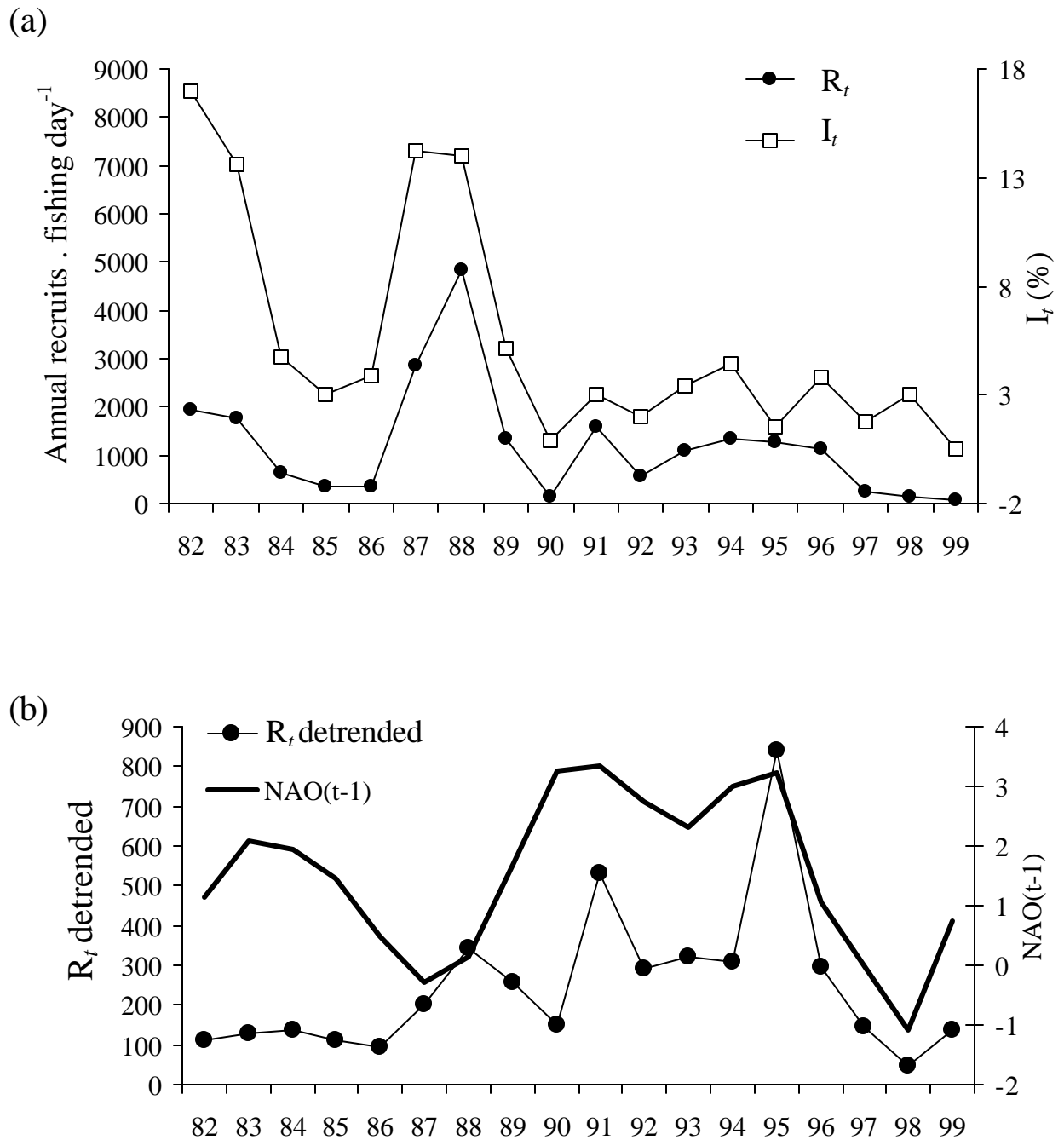
Figure 7. (a) Annual recruitment time series ( R_t ; line with circle) for whole Spanish trawling and the trend of annual percentage of hakes ( I_t ; line with square) caught respect to the grate total between 1982 and 1999. (b) Detrended annual recruitment time series ( R_t detrended) through removing I_t time series.
