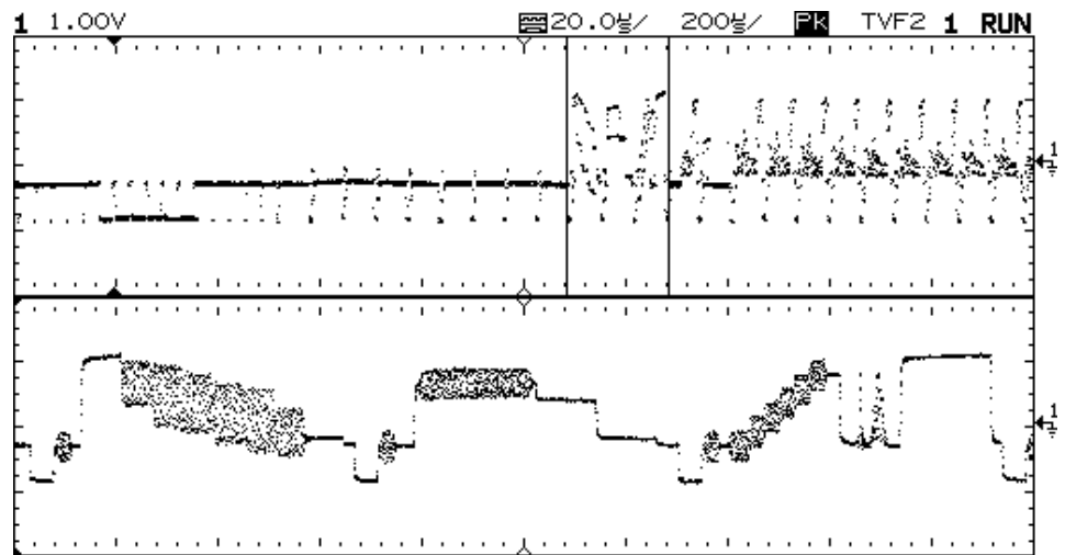
Second vertical interval windowed on the VITS
