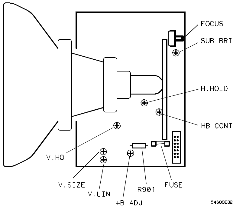
Display board adjustment locations
