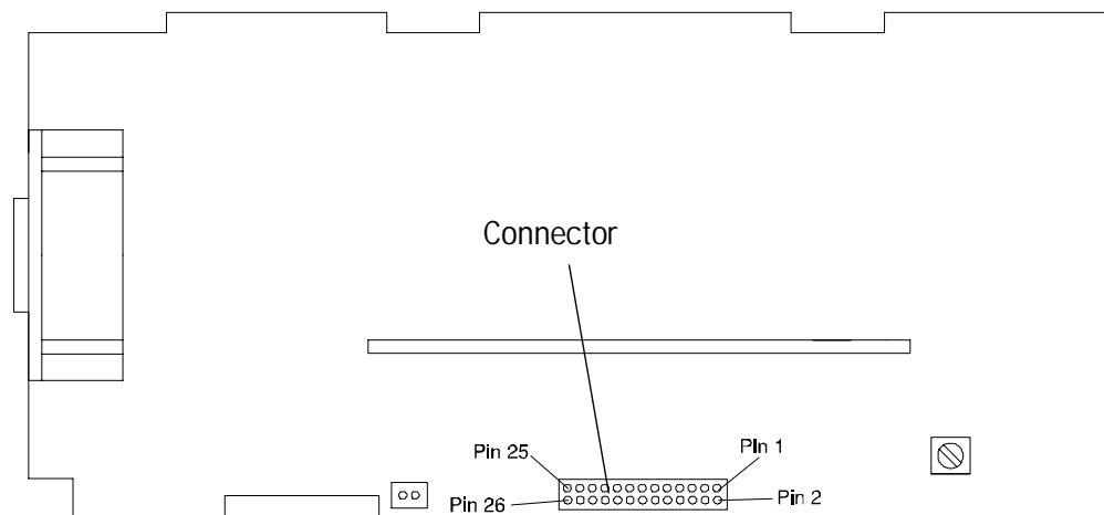
Low Voltage Power Supply connector pinout
