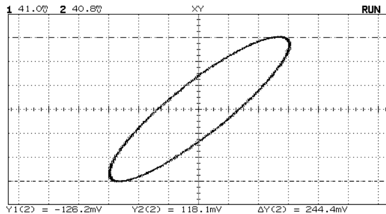
XY Display with Cursors On
