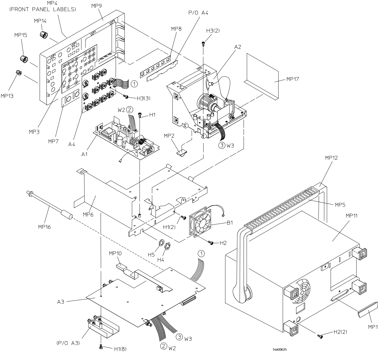
Exploded view of oscilloscope
