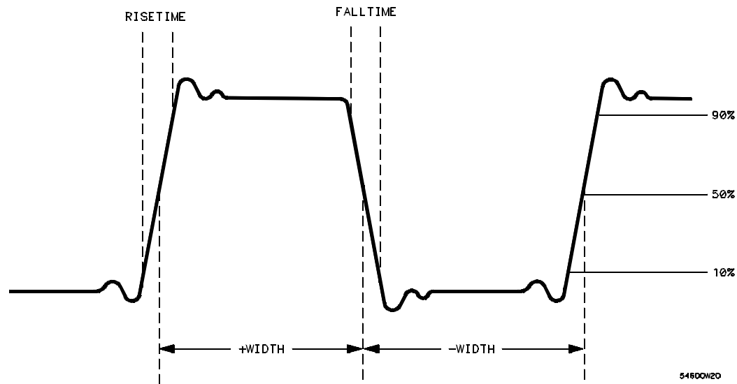
Time Measurement Points
