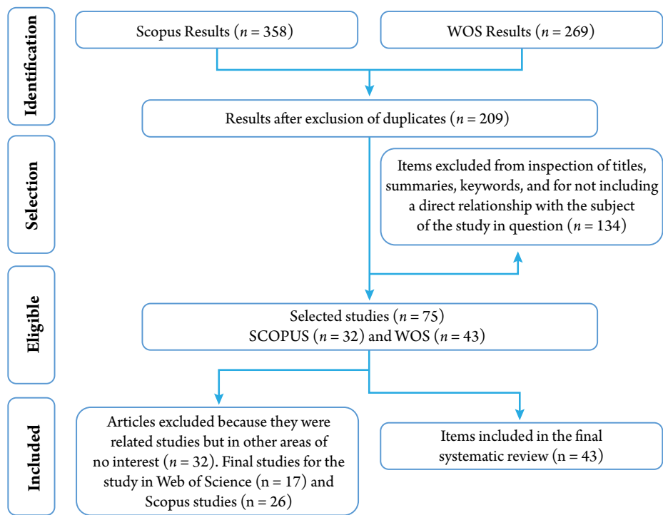
Figure 1. PRISMA Diagram
