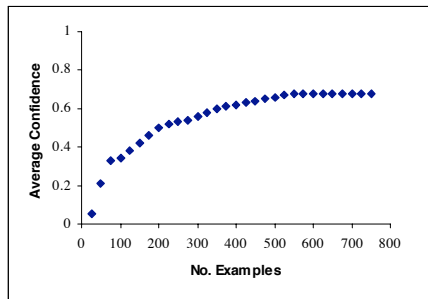
Accumulated predictive confidence
